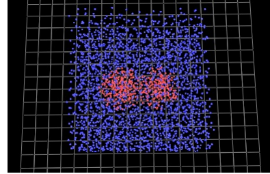
Figure 22: Close galaxies and negative mass distribution. m_+ = (1 \times 300) + (1 \times 300) = +600 , center1(-150,0,0), center2(+150,0,0), Positive mass is spread within R=180 . -m_- = -0.2 \times 3000 = -600 , negative mass distribution: -500 \leq x, y, z \leq +500
