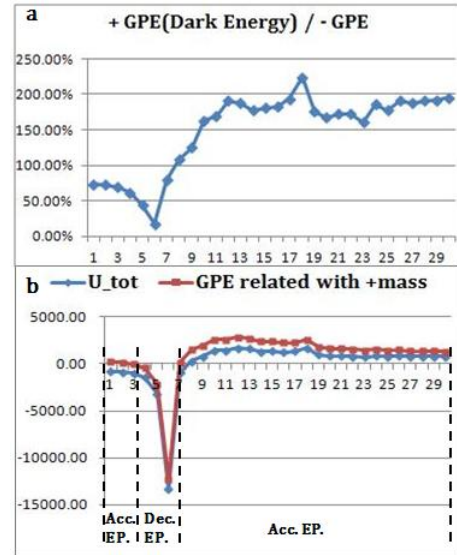
Figure 18: Fig.18-a. The ratio of +GPE to - GPE of distant galaxy. Fig.18-b. U_{tot} and GPE related with positive mass on distant galaxy. Note that GPE value related with positive mass changes from positive value to negative value, and to positive value again. This represents acceleration expansion - > deceleration expansion - > acceleration expansion of the universe.
